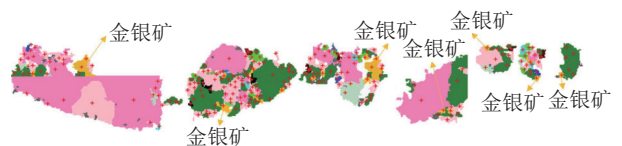
图 6 金银矿连生关系 Fig.6 Intergrowth relationship of electrum
